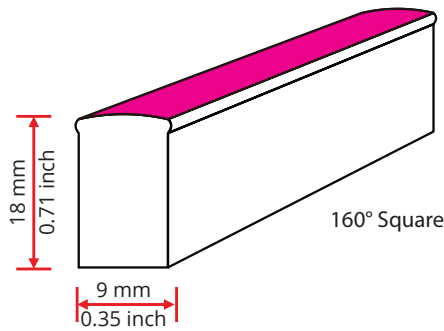
Light Profile
